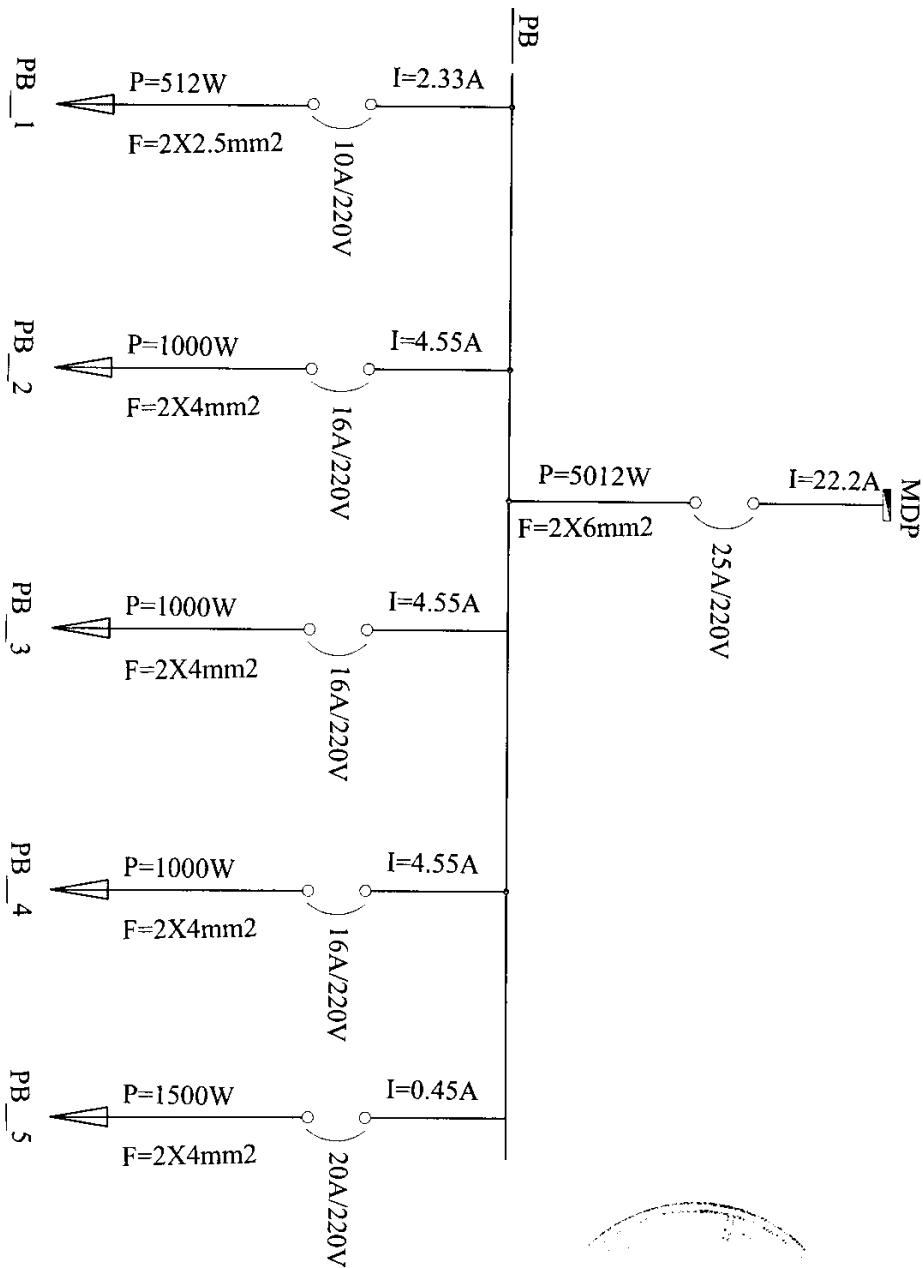
CIRCUIT DIAGRAM OF PB
